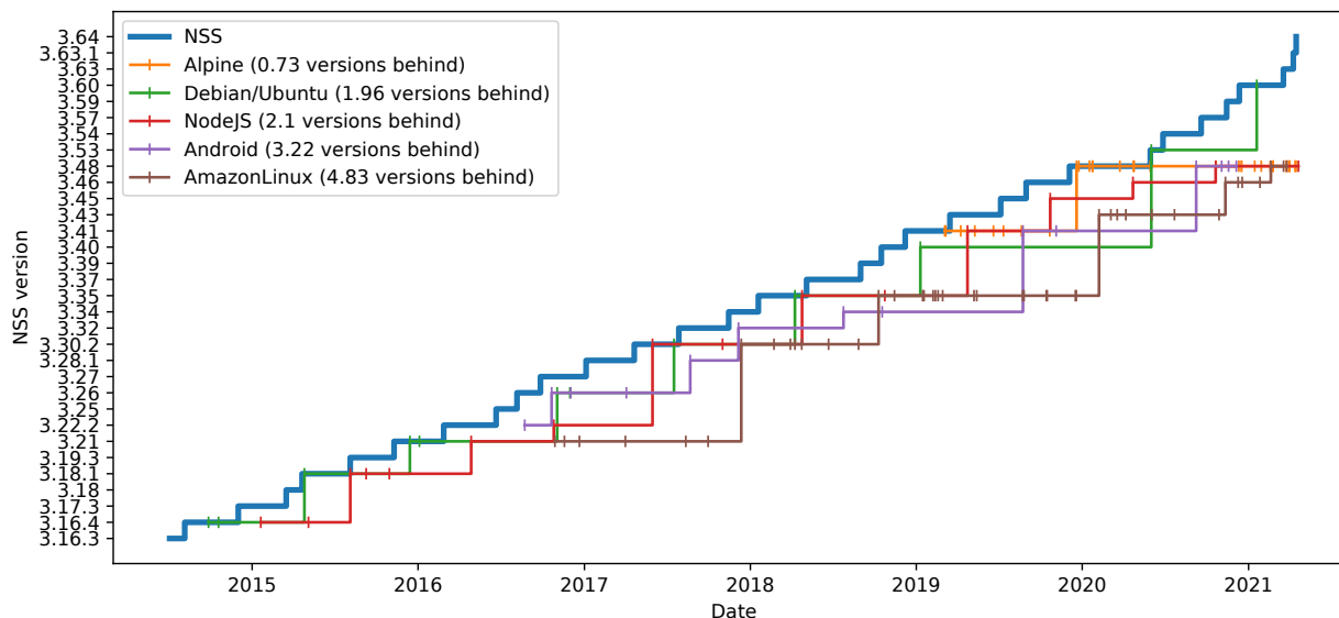
Figure 3.3: NSS derivative staleness —No derivative root stores match NSS’s update regularity. Alpine Linux maintains closest parity to NSS, while AmazonLinux, on average, lags more than four substantial versions behind.
