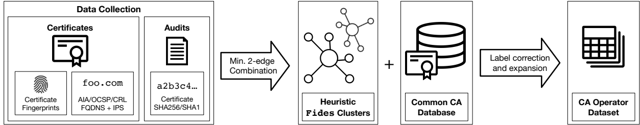
Figure 2.4: Fides—Integration of certificate- and audit-based data sources creates heuristic clusters that approximate shared CA certificate control. Combined with CCADB, Fides outputs a dataset of CA certificates and their operators.
